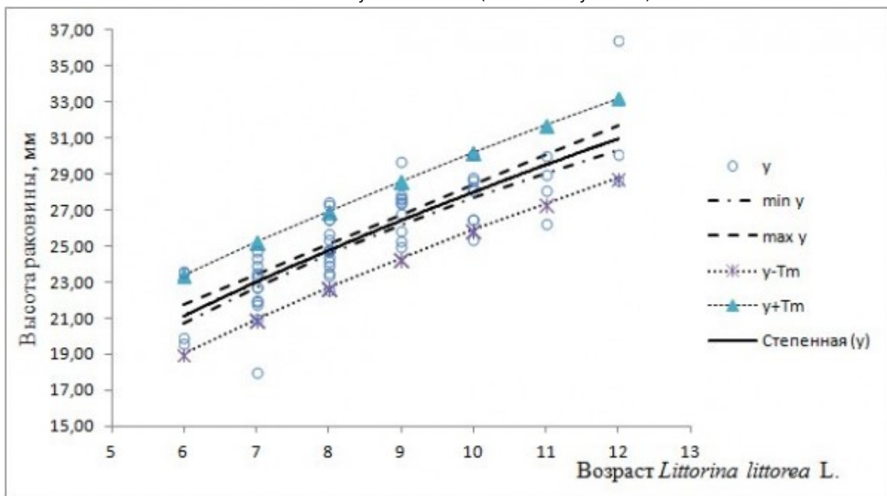
Fig. 4. The regression line ( y ), its confidence interval ( \min y ; \max y ) and forecast interval ( y-Tm ; y+Tm ) for the model y_i = 7.43x0.54 (the island Ryachkov)
